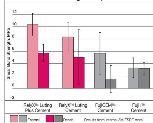
DATA: Shear Bond Strength Comparison
